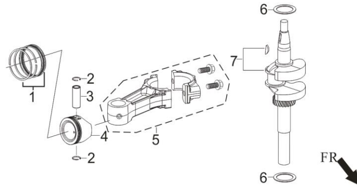
FIG.4 ROD,CRANKSHAFT CONNETING 曲柄连杆组件(E04)
