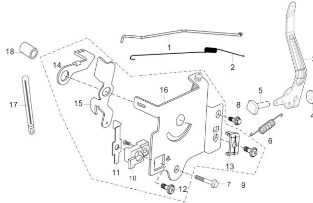
FIG.13 CONTROL ASSY, THROTTLE 油门操纵部件 ( E13 )
