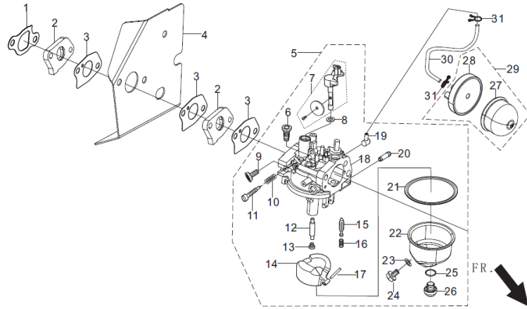
FIG.8 CARBURETOR ASSY. 化油器部件 ( E08 )
