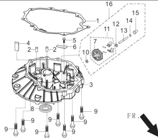
FIG.3 COVER SUBASSEMBLY, CRANKCASE / GEAR ASSY, GOVERNOR 曲轴箱盖部件 + 调速齿轮部件(E03)
