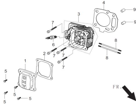
FIG.1 HEAD SUBASSEMBLY, CYLINDER / PLUG, SPARK 气缸头部件/火花塞 (E01)
