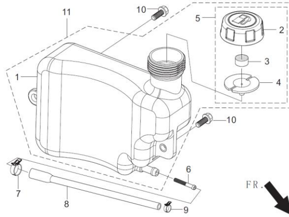
FIG.11 TANK, FUEL 油箱 ( E11 )
