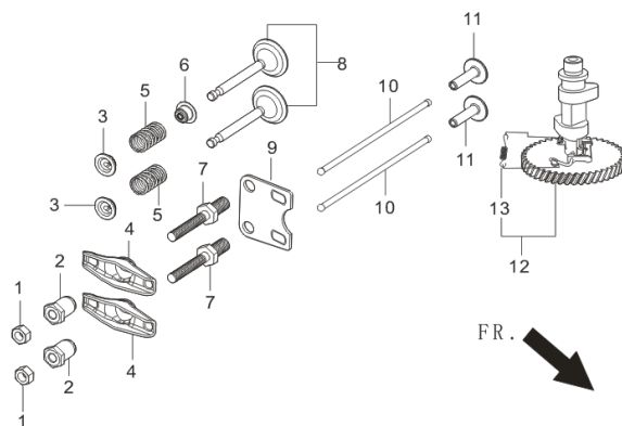
FIG.5 TRAIN,VALVE / CAMSHAFT SUBASSEMBLY 配气机构组件/凸轮轴 ( E05 )
